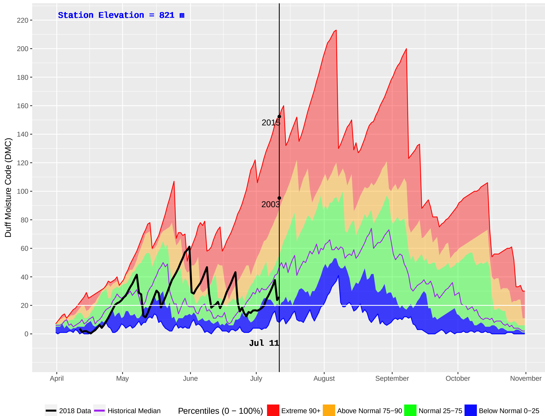
AKOKLI CREEK (838) : Historical (2003–2016) and Current (2018) Noon Duff Moisture Code (DMC)
