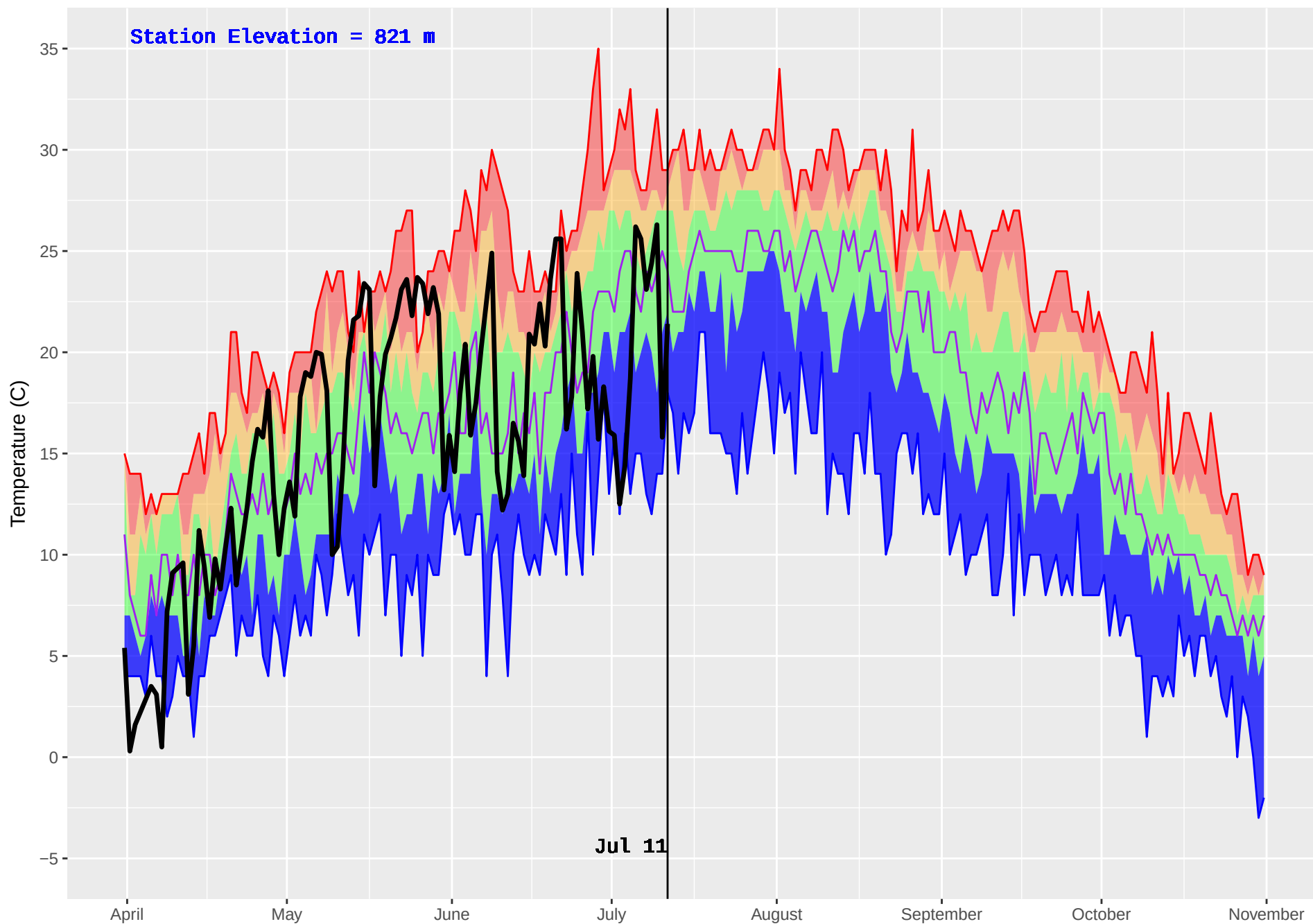
AKOKLI CREEK (838) : Historical (2003–2016) and Current (2018) Noon Temperature
