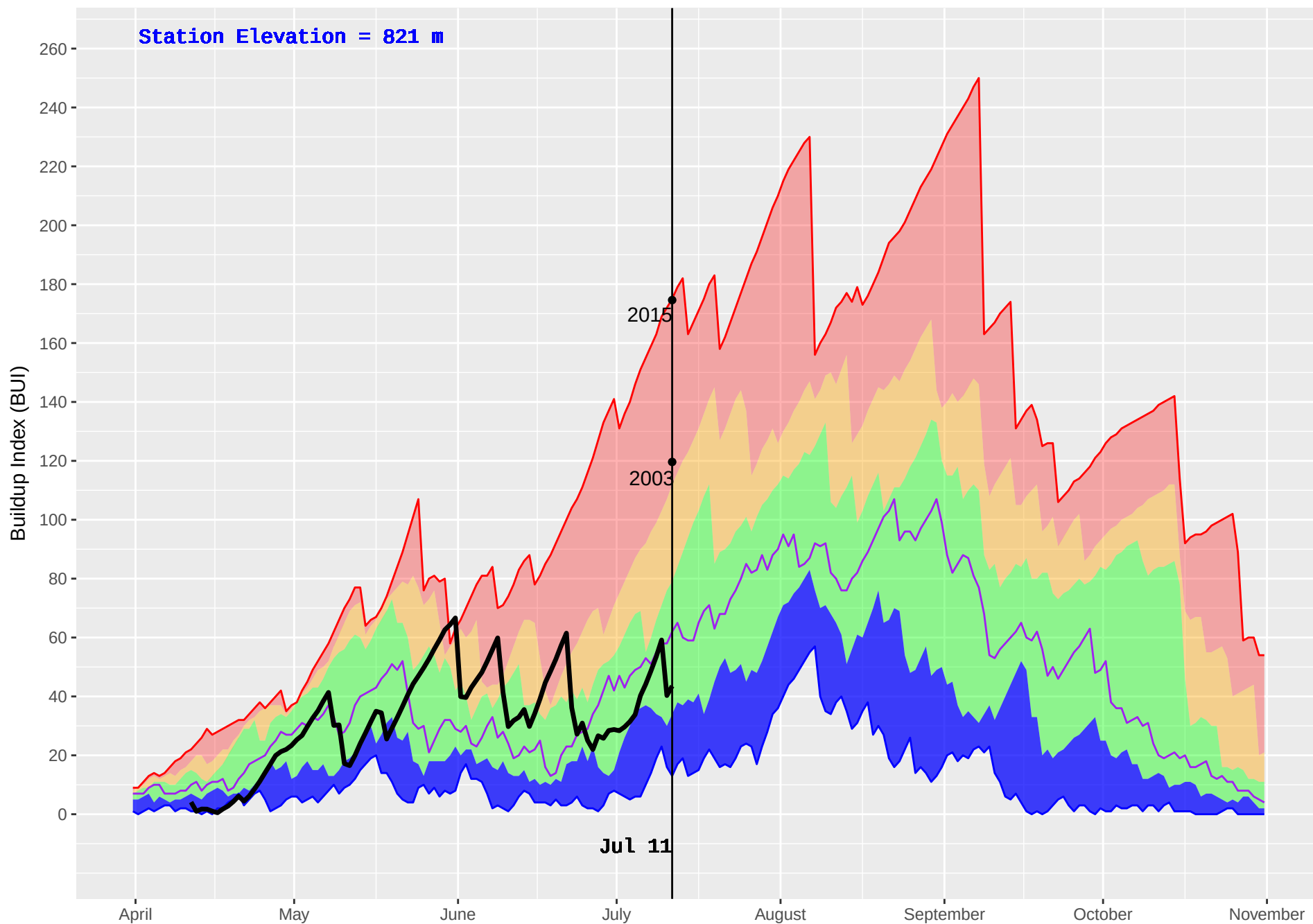
AKOKLI CREEK (838) : Historical (2003–2016) and Current (2018) Noon Buildup Index (BUI)
