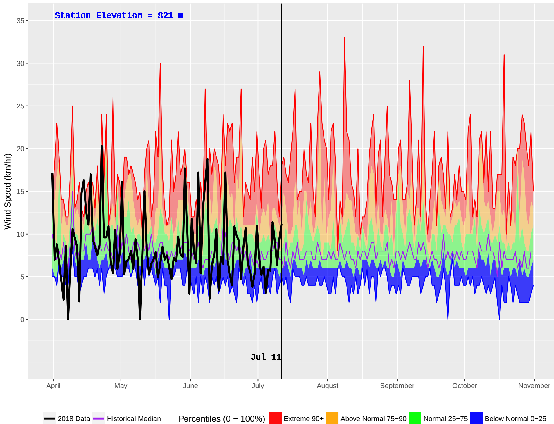
AKOKLI CREEK (838) : Historical (2003–2016) and Current (2018) Noon Wind Speed
